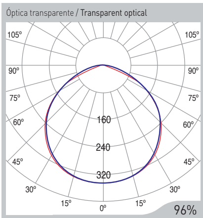
Duris E5 120°
