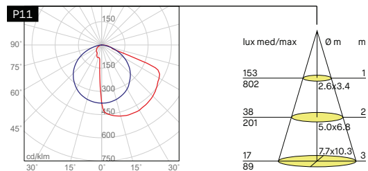
P11 + BARRA/STRIP/10 + 80300/C
