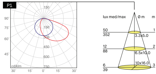
P1 + 2xBARRA/STRIP/3E + 2x70092/C
