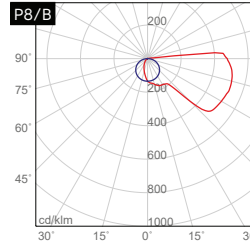
P8/B + BARRA/STRIP/10 + 80300/C
