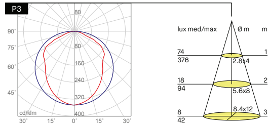
P3 + 2xBARRA/STRIP/3E + 2x70092/C
